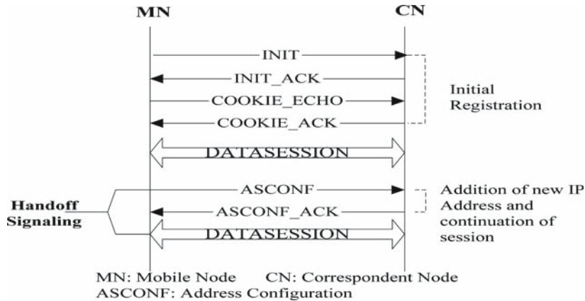
Figure 3. Sctp-based mobility management.
